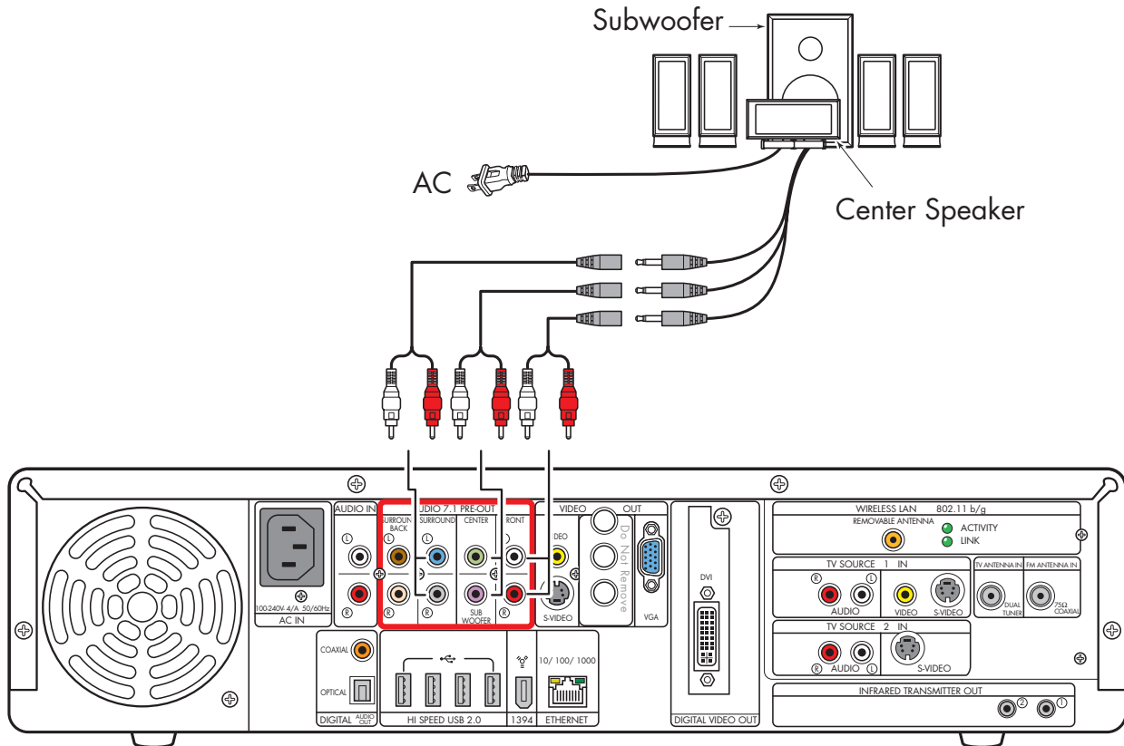
Typical 5.1 powered speaker installation
